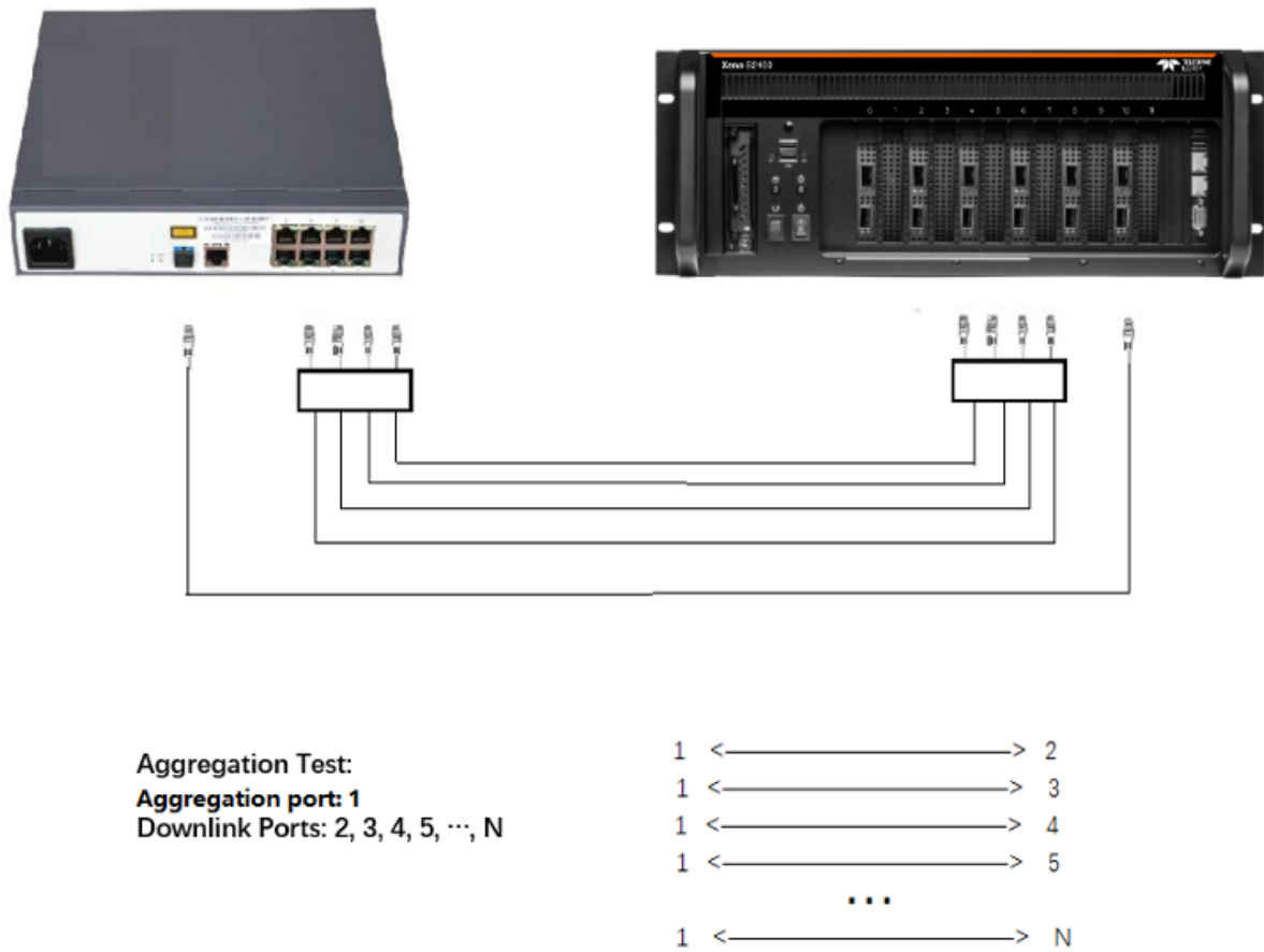
Fig. 15.1: Aggregation Test Case diagram
