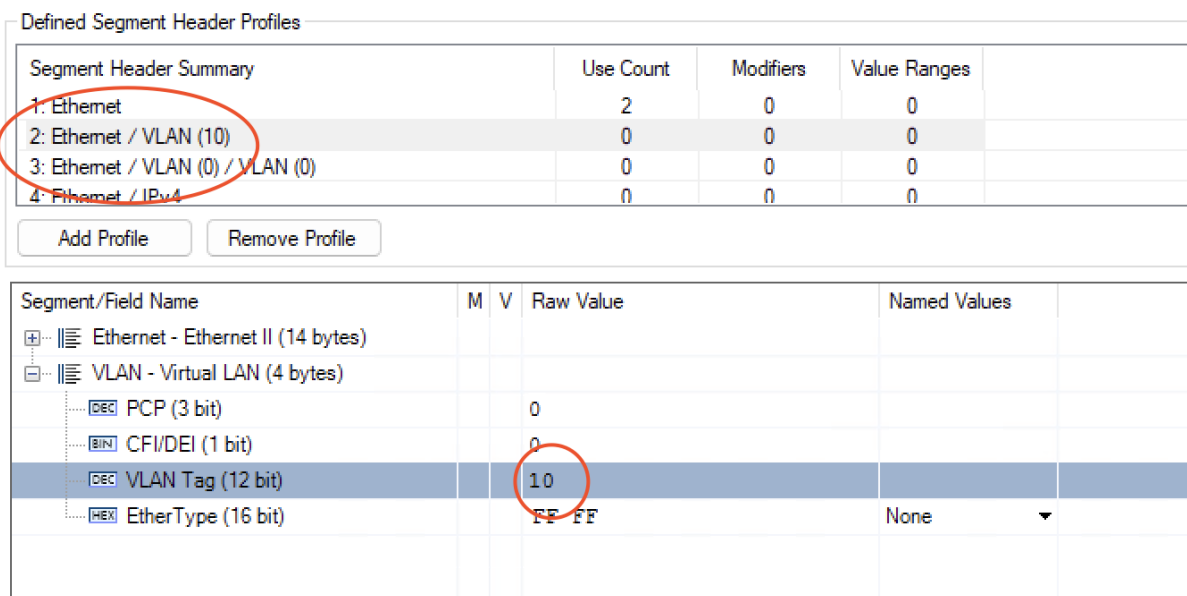
Fig. 4.8: VLAN tag 10 profile
