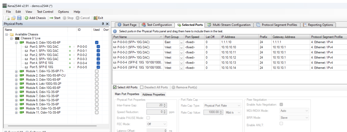
Fig. 15.9: Assign one port to a group and others the other group. Assign L3 profile to ports
