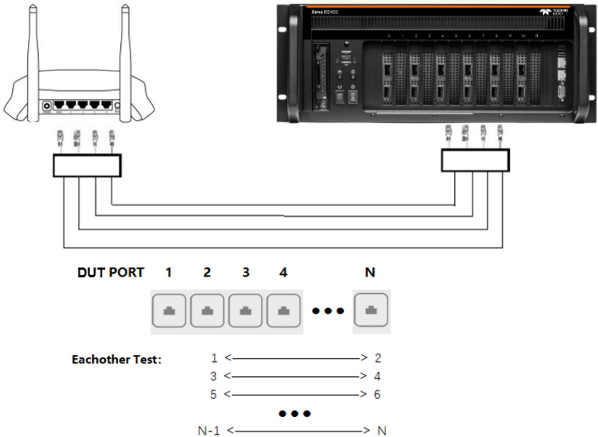
Fig. 15.4: Each-Other Test Case diagram
