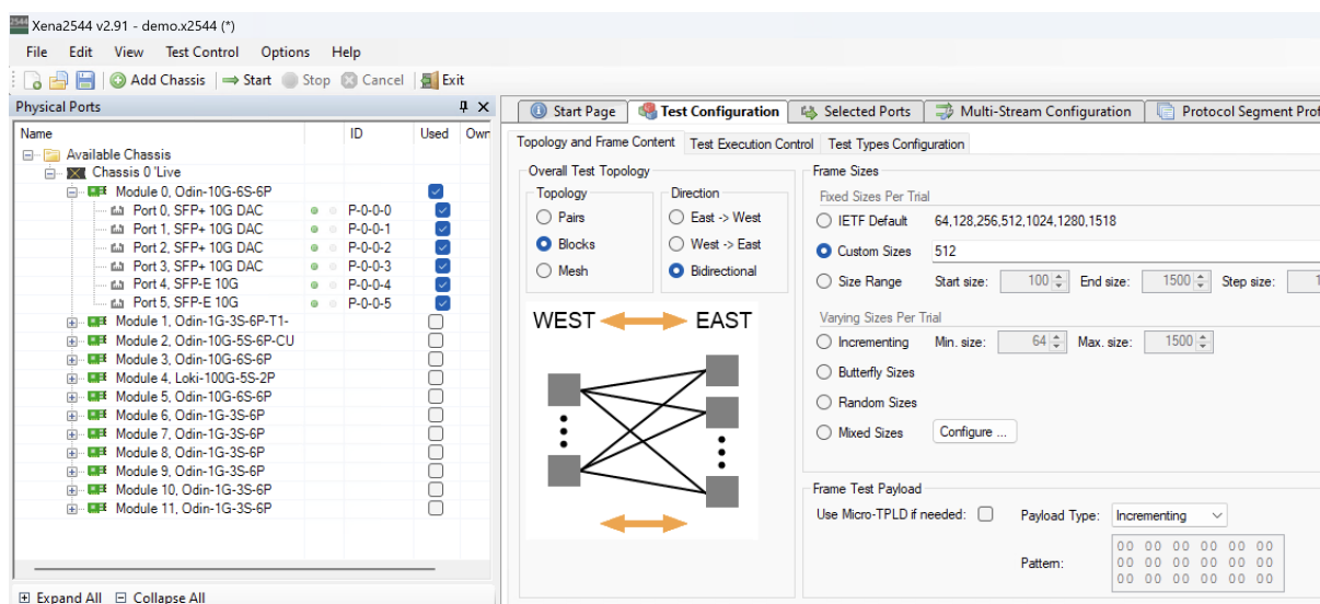
Fig. 15.8: Set topology to Block + Bidirectional
