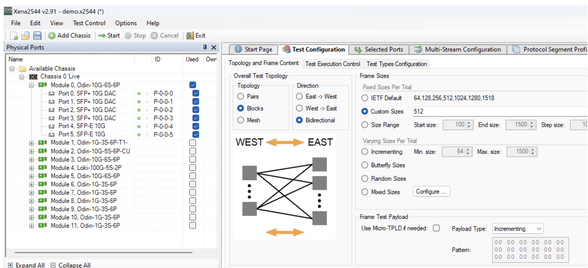
Fig. 15.2: Set topology to Block + Bidirectional
