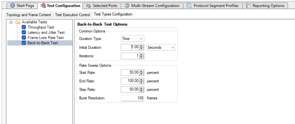
Fig. 7.7: Back-to-back test options
